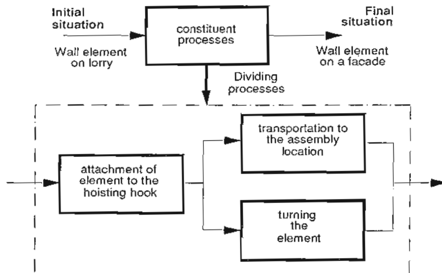
Figure 2. Transportation of wall elements.
